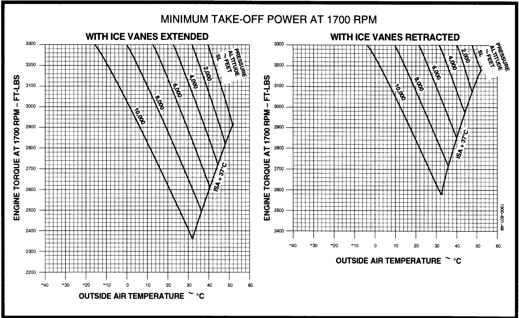
FIGURE 12.—Minimum Takeoff Power at 1700 RPM.
