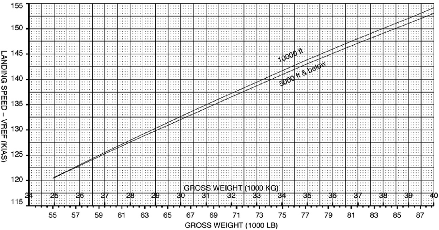
Landing Speed - Flaps at 45 Degrees/Slats Extended
